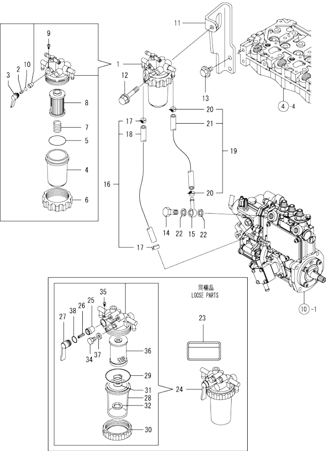
Fig.13. FUEL LINE
