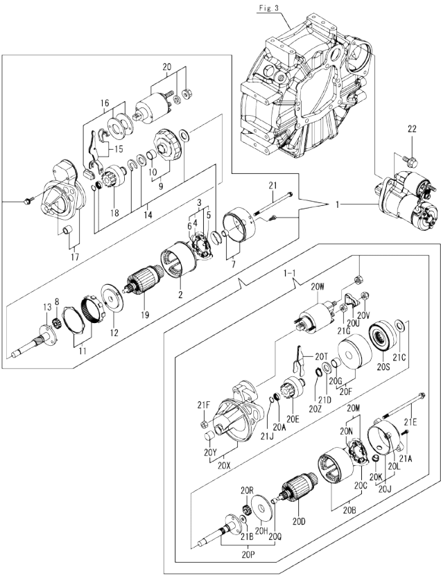
0CW10-M47000 3TNM68-HGEP Fig.14. STARTING MOTOR
