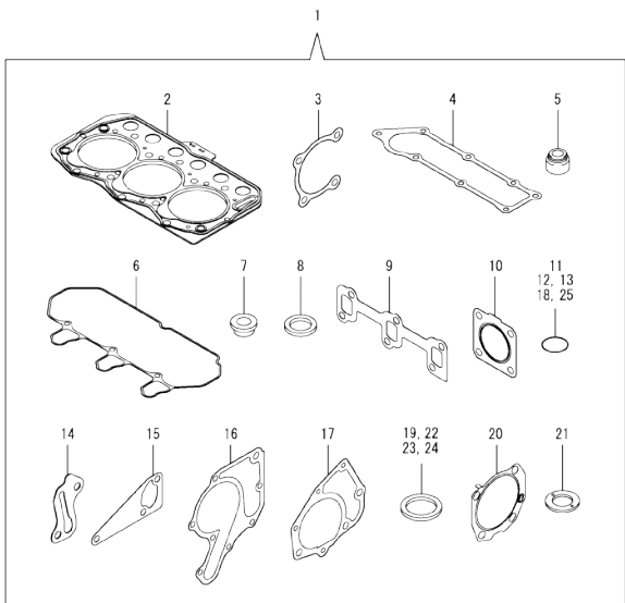
0CW10-M47000 3TNM68-HGEP Fig.16. GASKET SET
